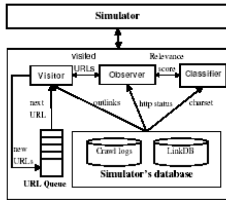
Figure 2. Architecture of the Web Crawling Simulator
