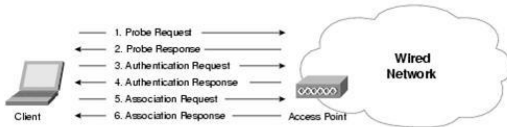
Fig:1 Showing the transactions of 802.11 client authentication process
