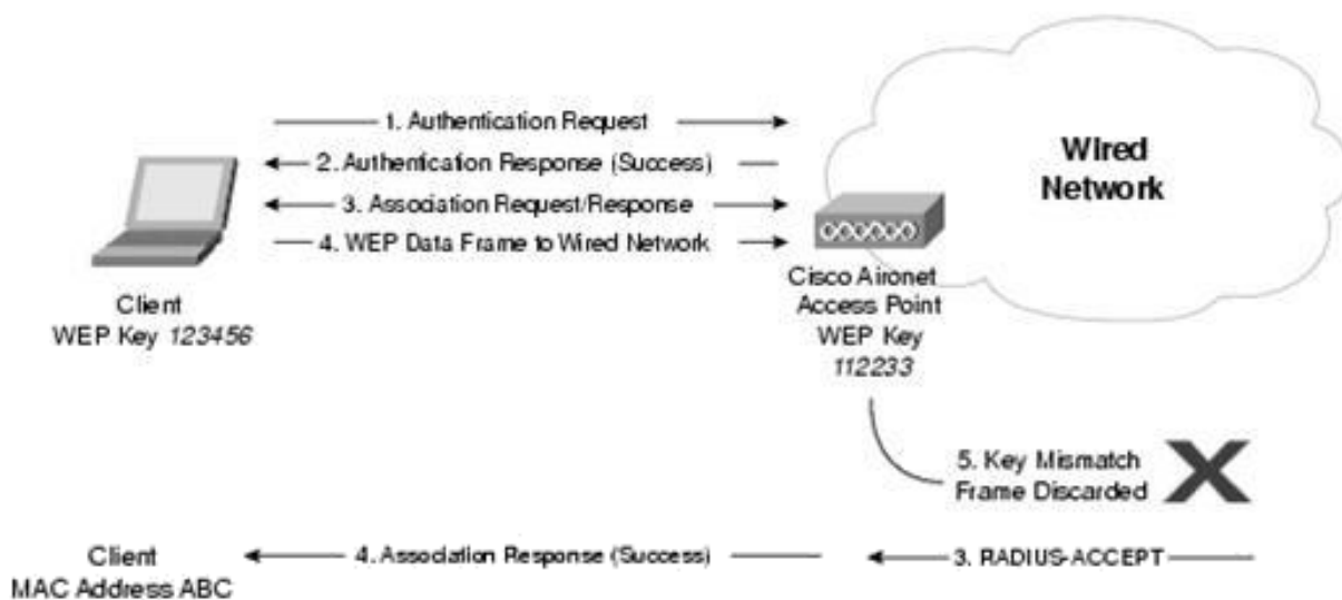
Fig 3: Shared Key Authentication
